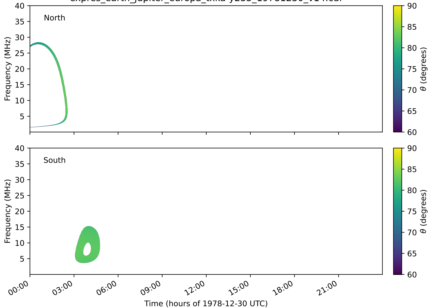
expres_earth_jupiter_europa_txka-y235_19781230_v14.cdf
