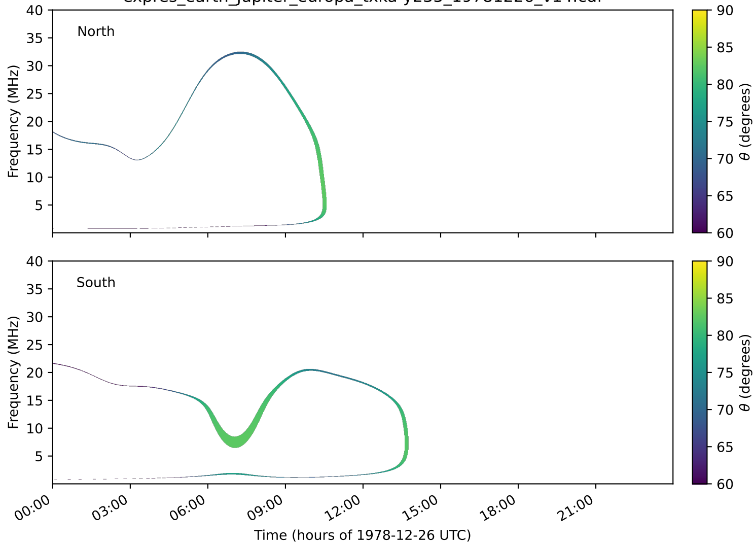
expres_earth_jupiter_europa_txka-y235_19781226_v14.cdf
