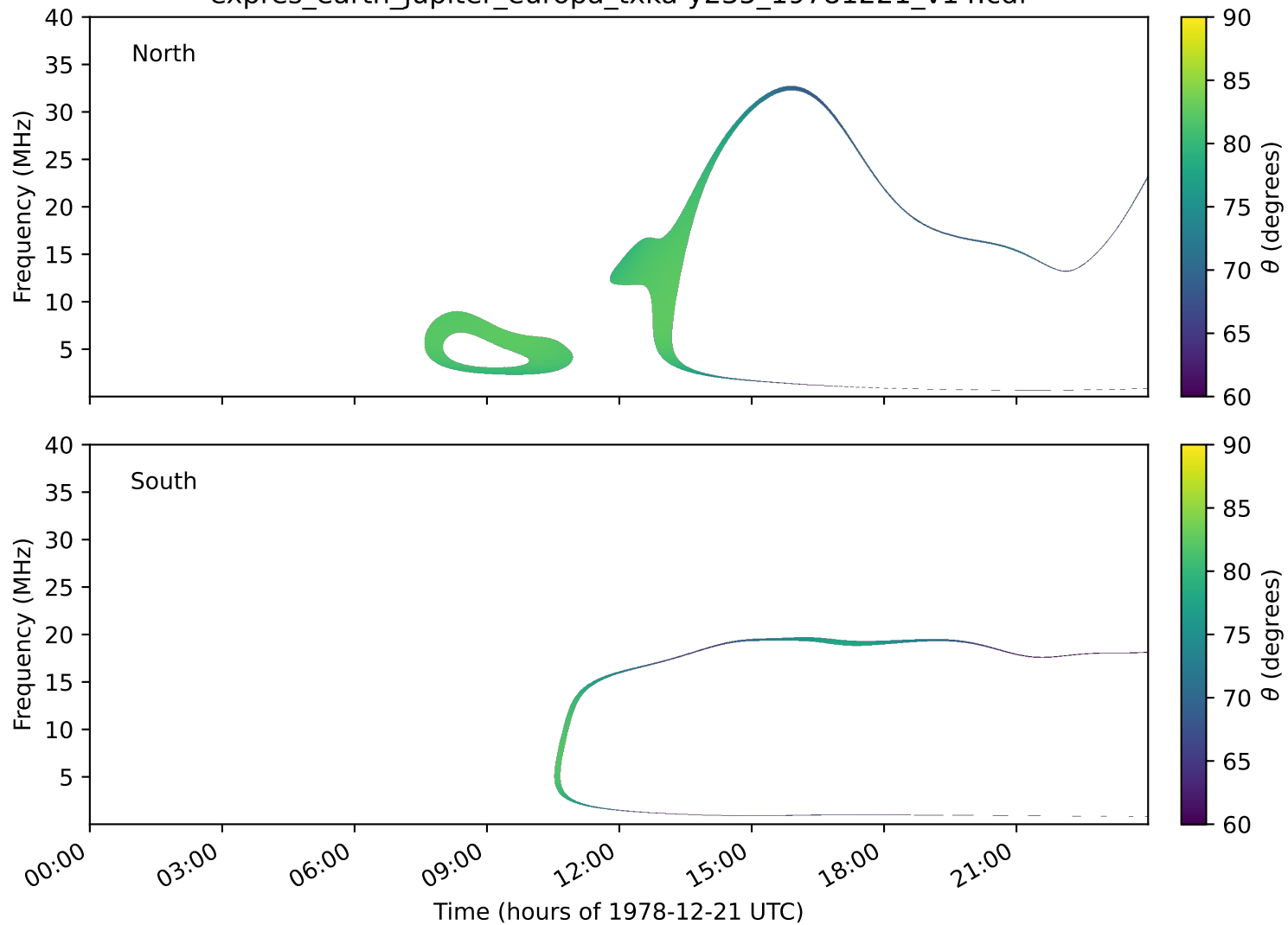
expres_earth_jupiter_europa_txka-y235_19781221_v14.cdf
