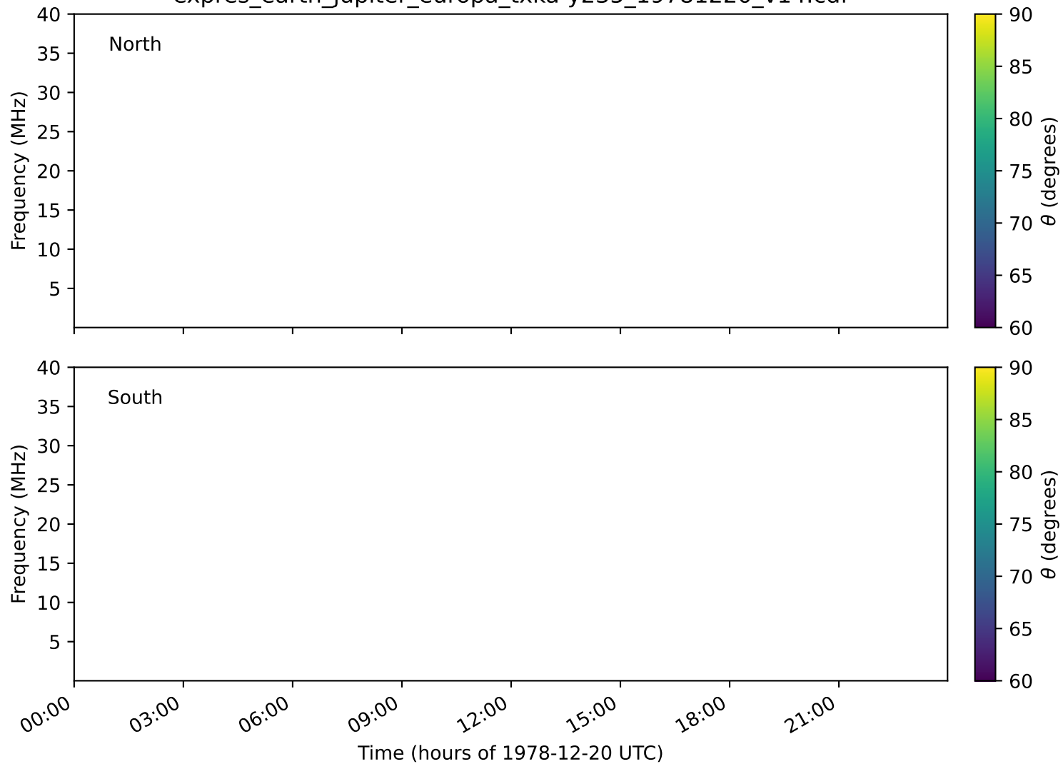
expres_earth_jupiter_europa_txka-y235_19781220_v14.cdf
