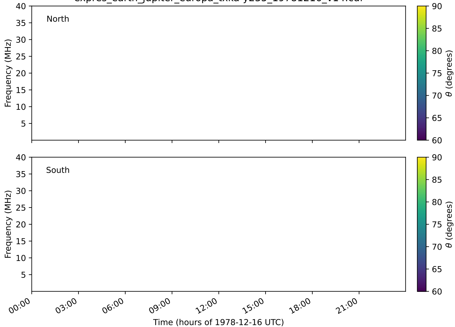
expres_earth_jupiter_europa_txka-y235_19781216_v14.cdf
