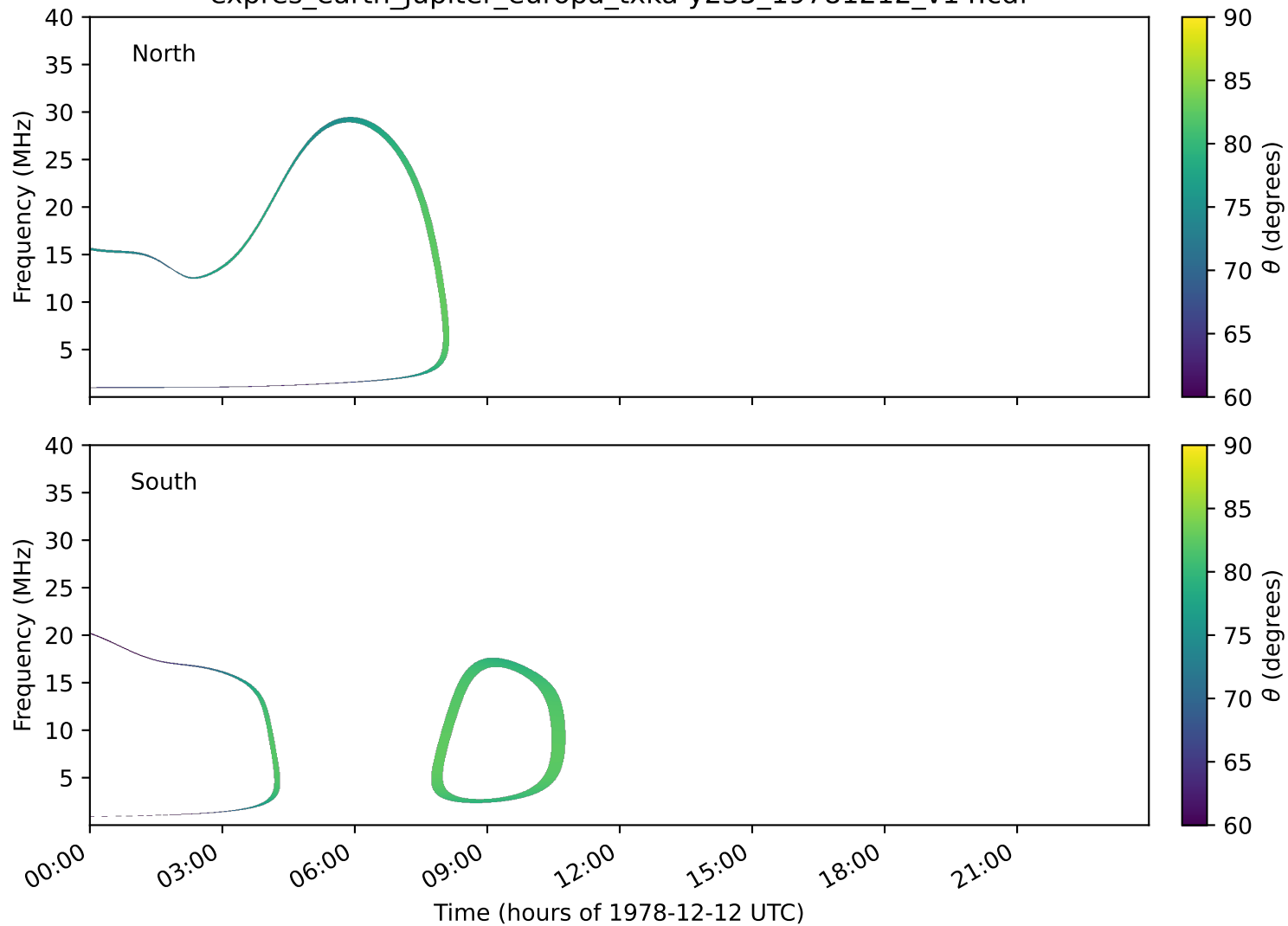
expres_earth_jupiter_europa_txka-y235_19781212_v14.cdf
