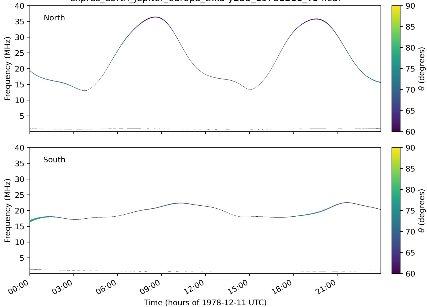
expres_earth_jupiter_europa_txka-y235_19781211_v14.cdf
