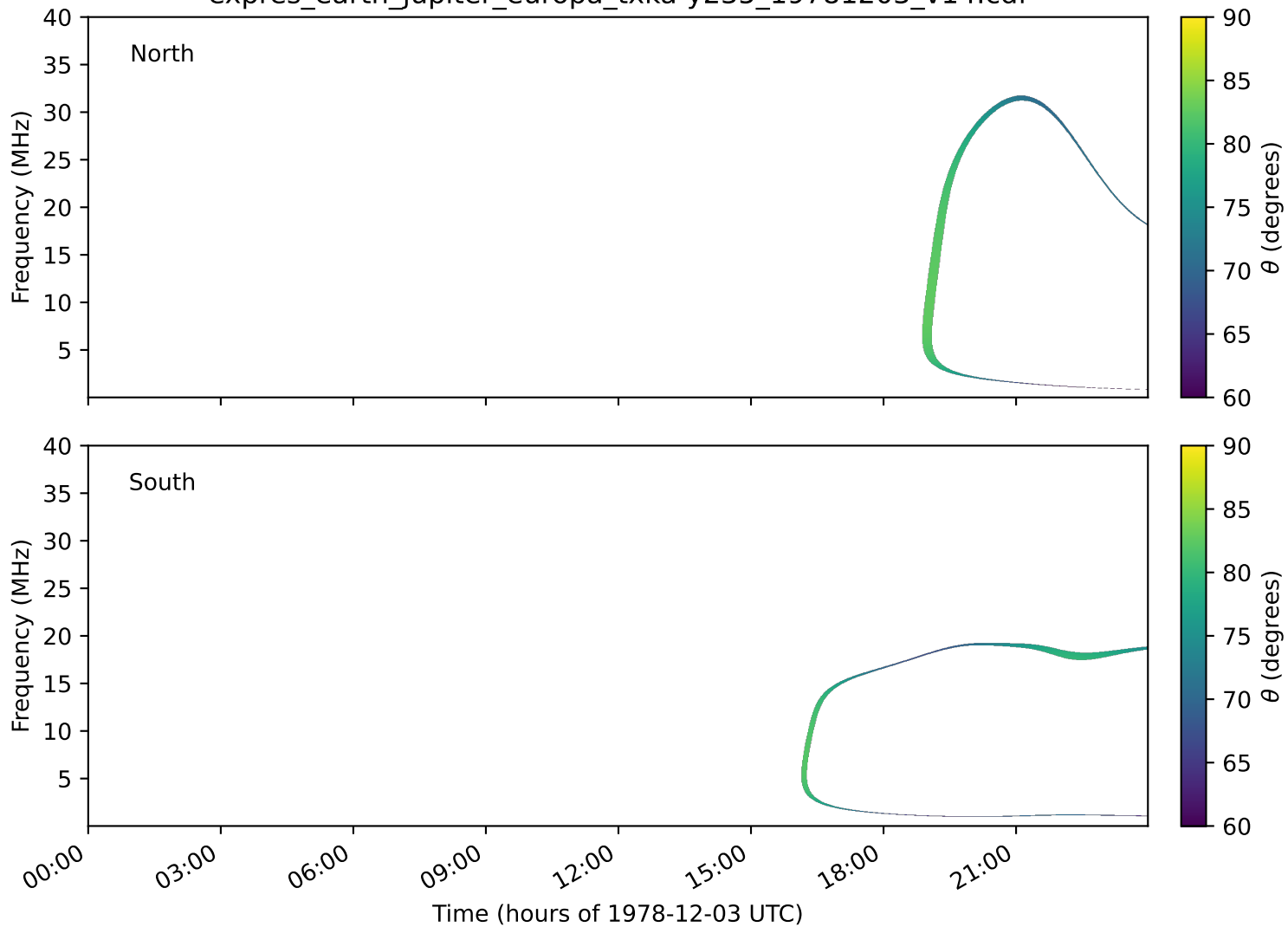
expres_earth_jupiter_europa_txka-y235_19781203_v14.cdf
