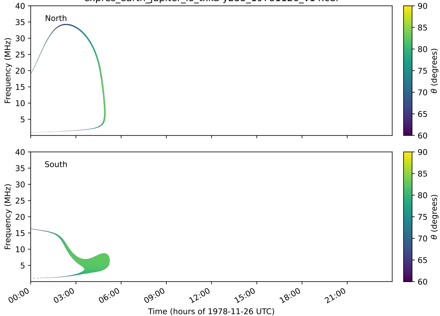
expres_earth_jupiter_io_txka-y235_19781126_v14.cdf
