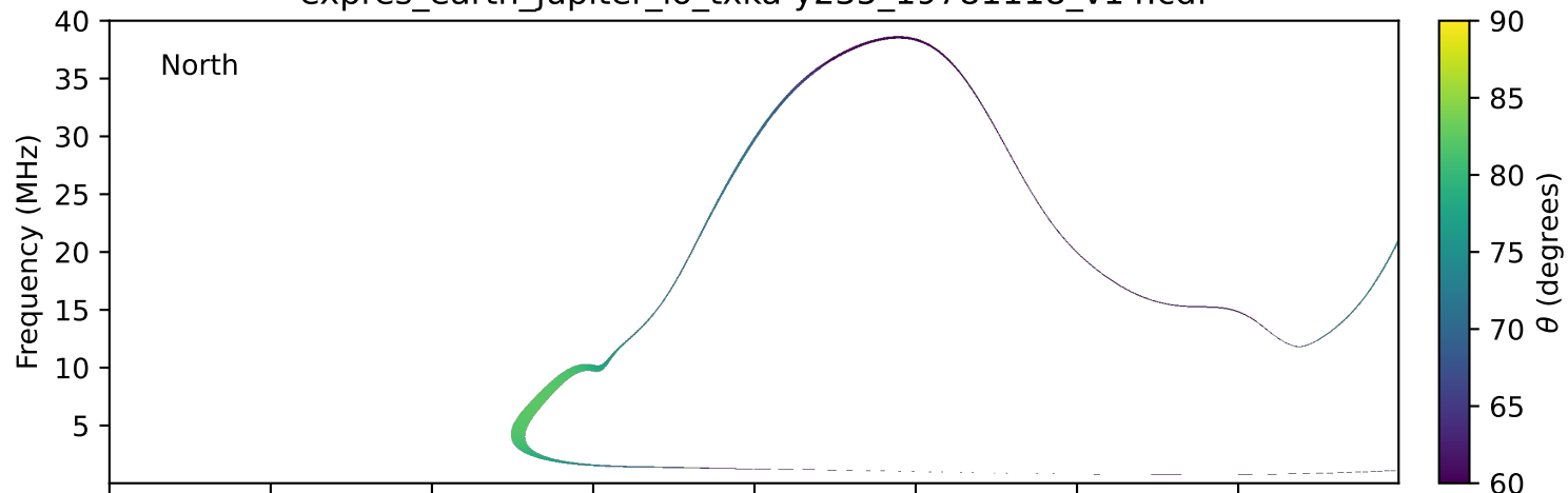
expres_earth_jupiter_io_txka-y235_19781118_v14.cdf
