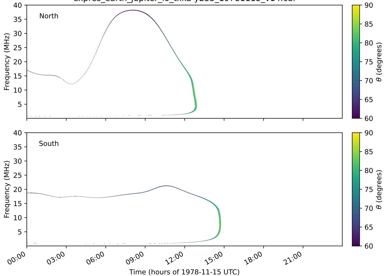
expres_earth_jupiter_io_txka-y235_19781115_v14.cdf
