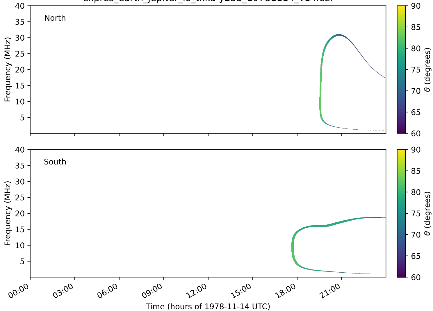
expres_earth_jupiter_io_txka-y235_19781114_v14.cdf
