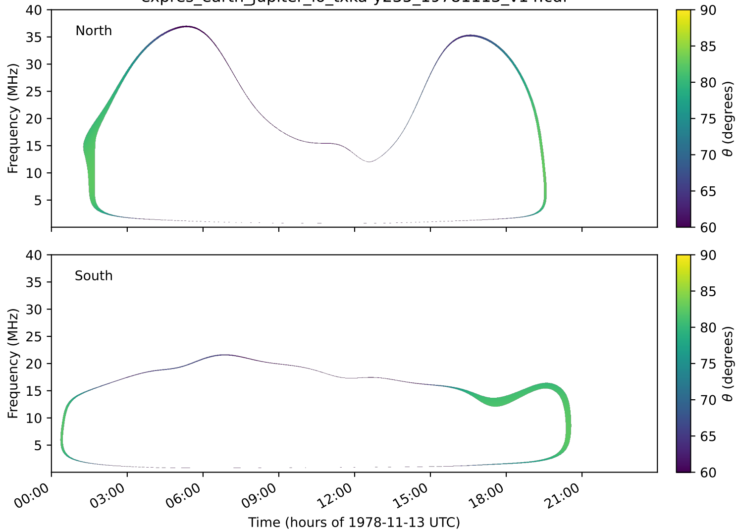
expres_earth_jupiter_io_txka-y235_19781113_v14.cdf
