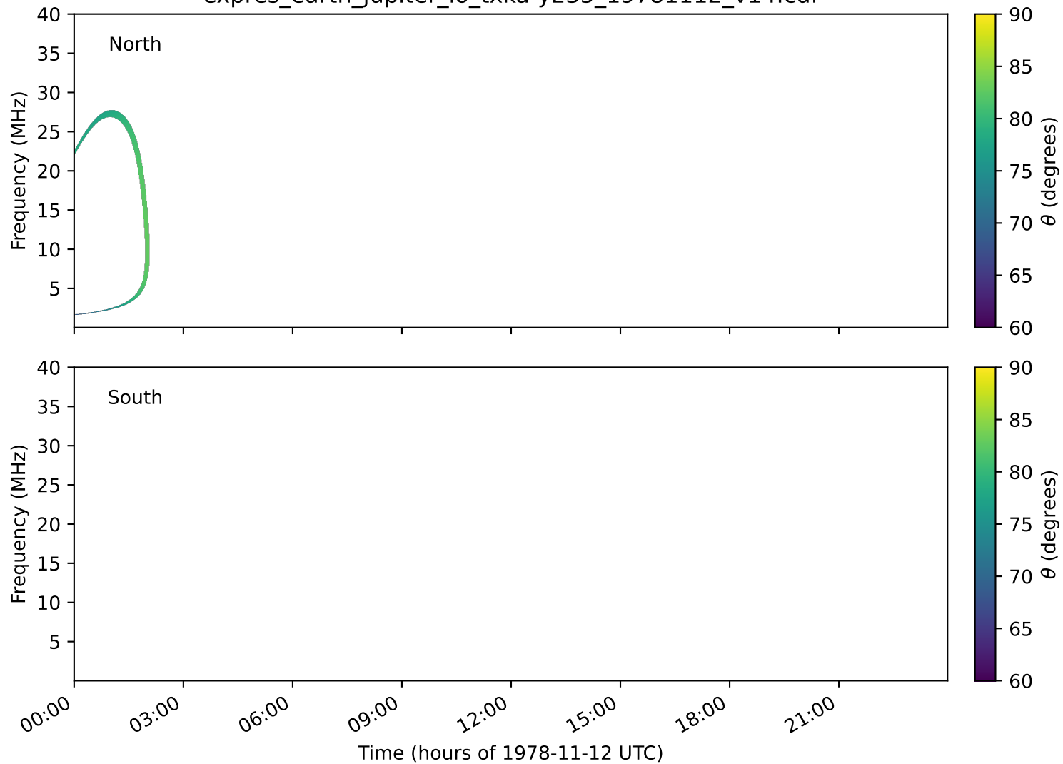
expres_earth_jupiter_io_txka-y235_19781112_v14.cdf
