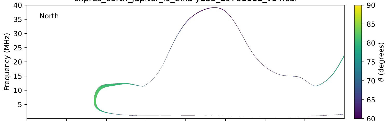
expres_earth_jupiter_io_txka-y235_19781111_v14.cdf
