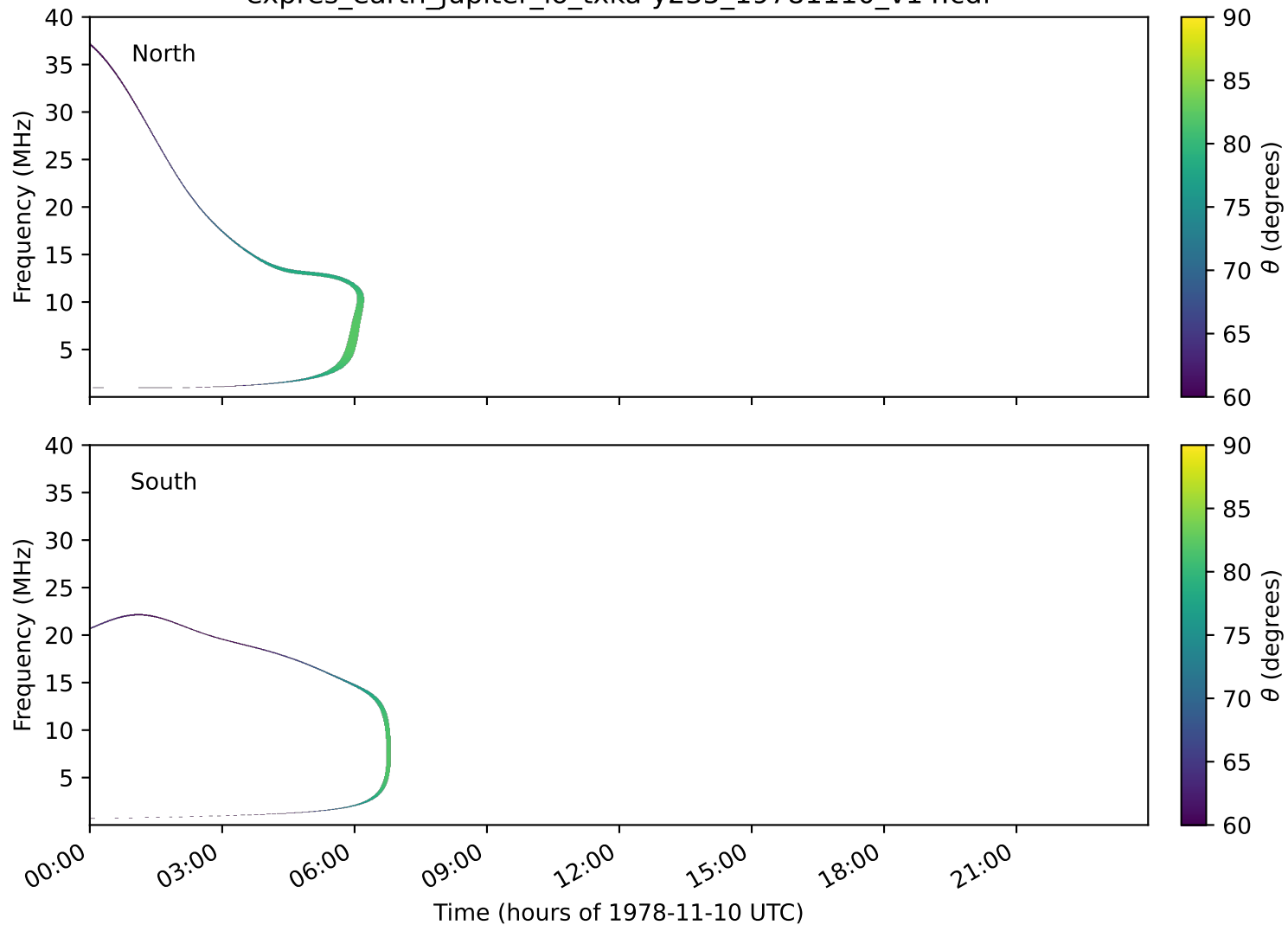
expres_earth_jupiter_io_txka-y235_19781110_v14.cdf
