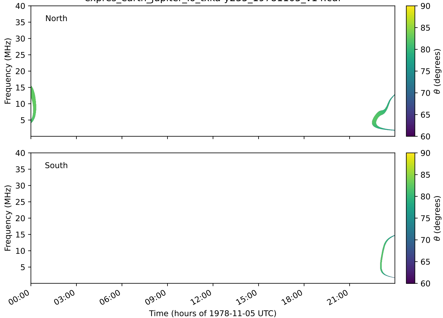
expres_earth_jupiter_io_txka-y235_19781105_v14.cdf
