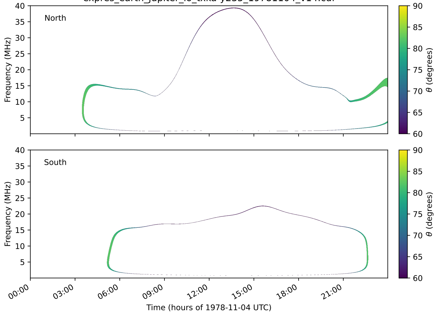
expres_earth_jupiter_io_txka-y235_19781104_v14.cdf
