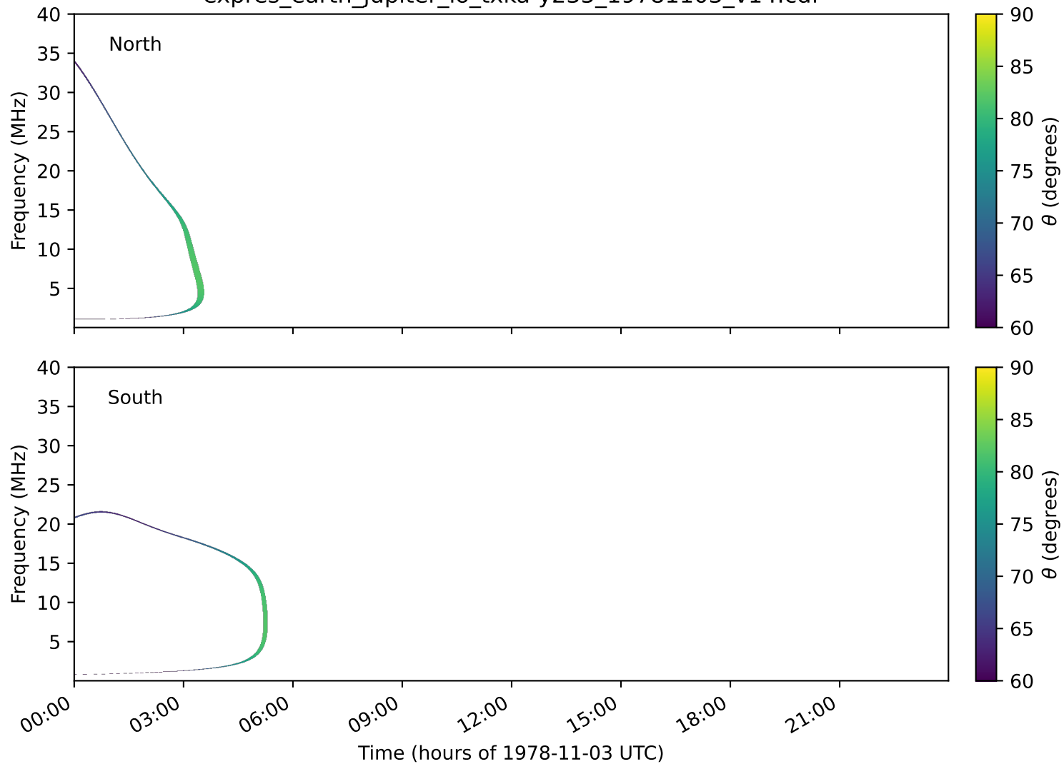
expres_earth_jupiter_io_txka-y235_19781103_v14.cdf
