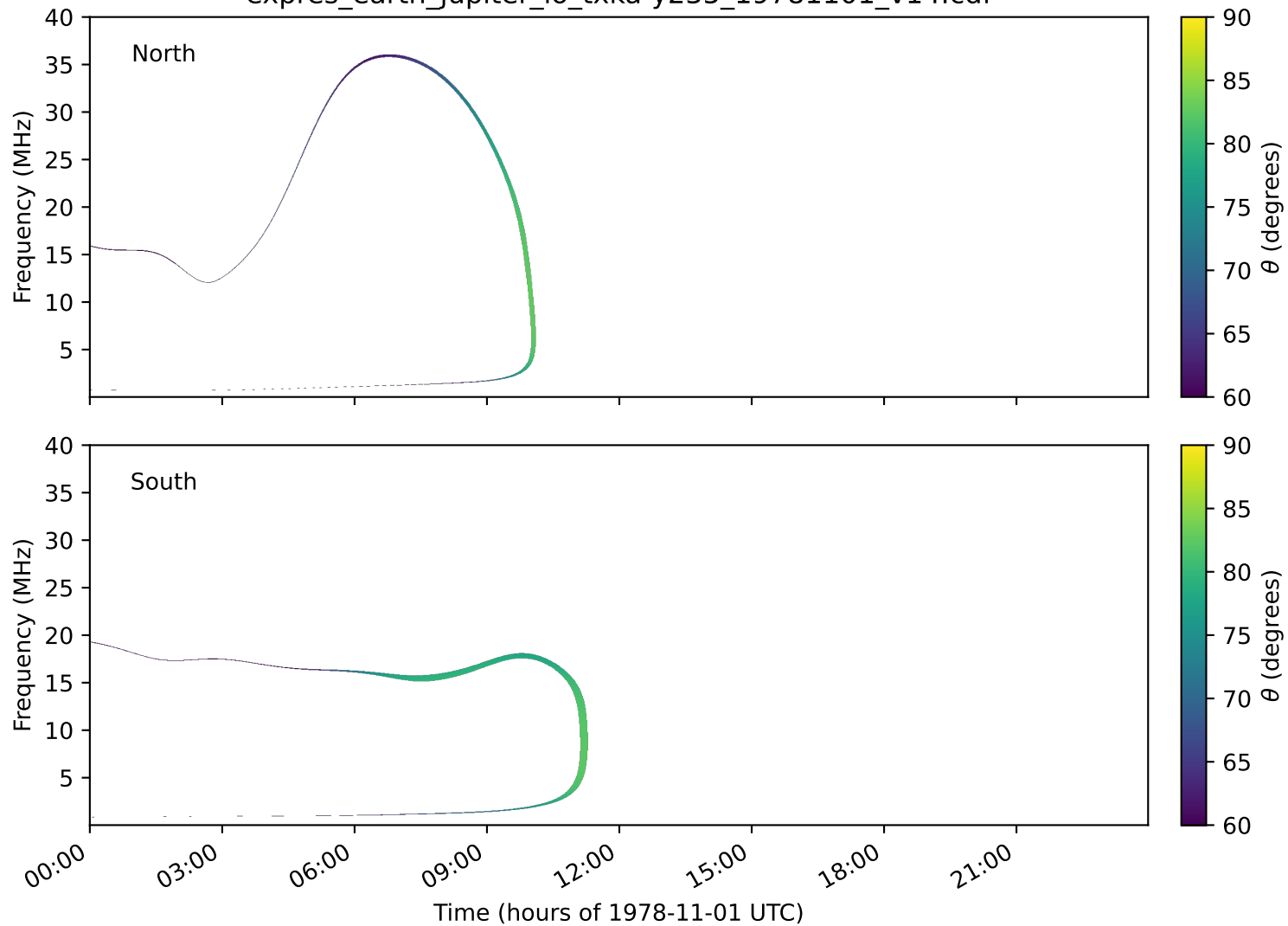
expres_earth_jupiter_io_txka-y235_19781101_v14.cdf
