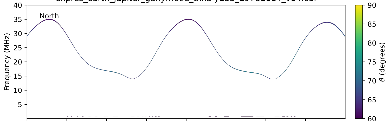
expres_earth_jupiter_ganymede_txka-y235_19781114_v14.cdf
