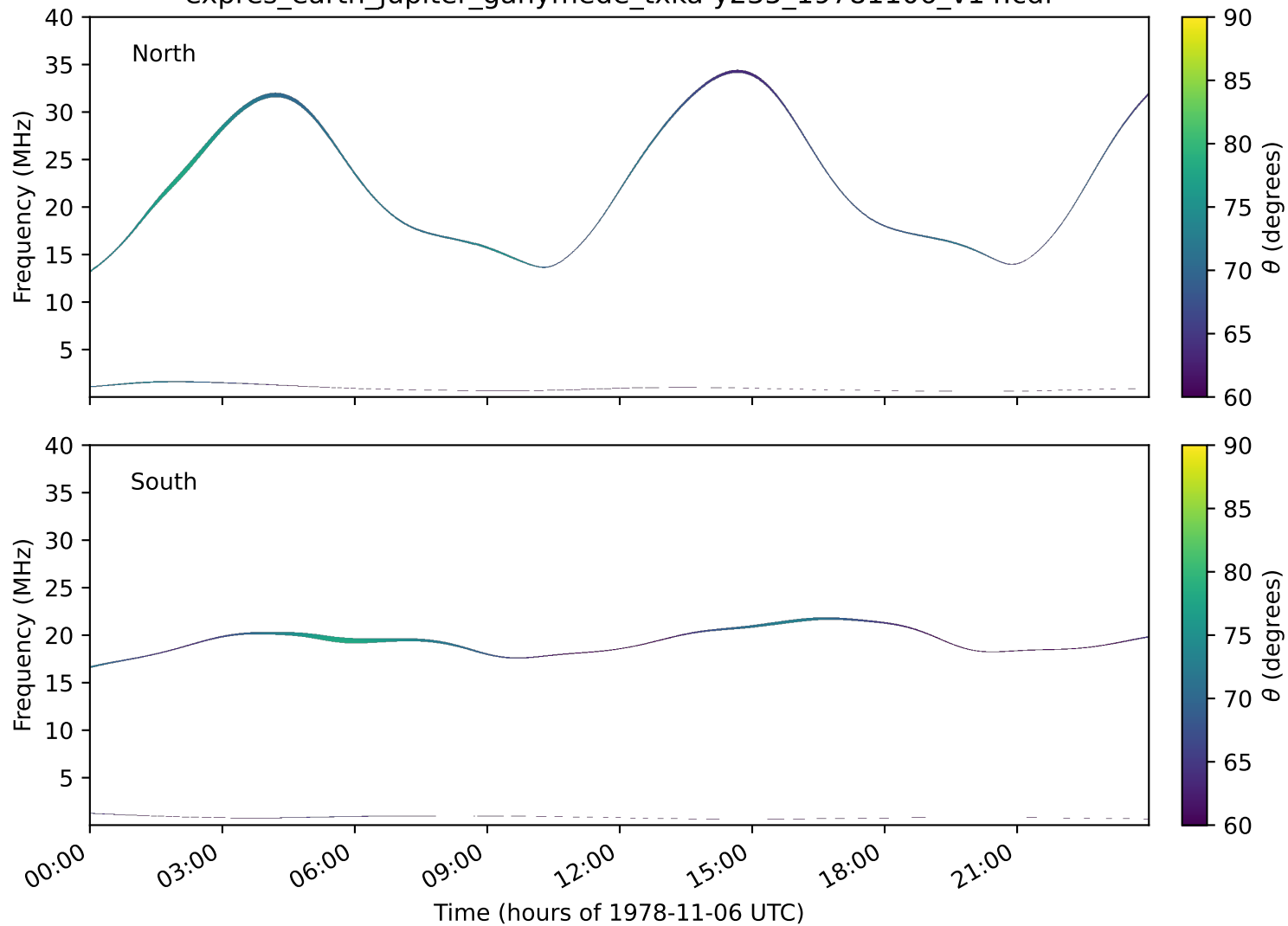
expres_earth_jupiter_ganymede_txka-y235_19781106_v14.cdf
