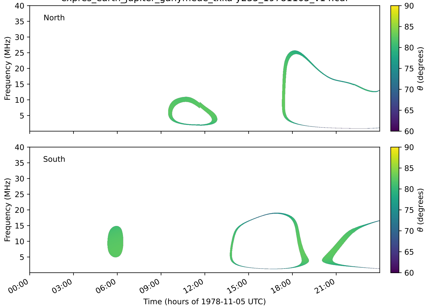
expres_earth_jupiter_ganymede_txka-y235_19781105_v14.cdf
