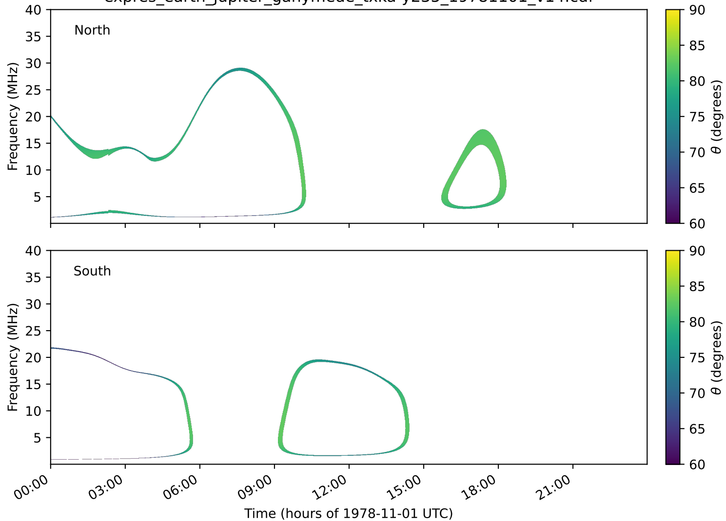
expres_earth_jupiter_ganymede_txka-y235_19781101_v14.cdf
