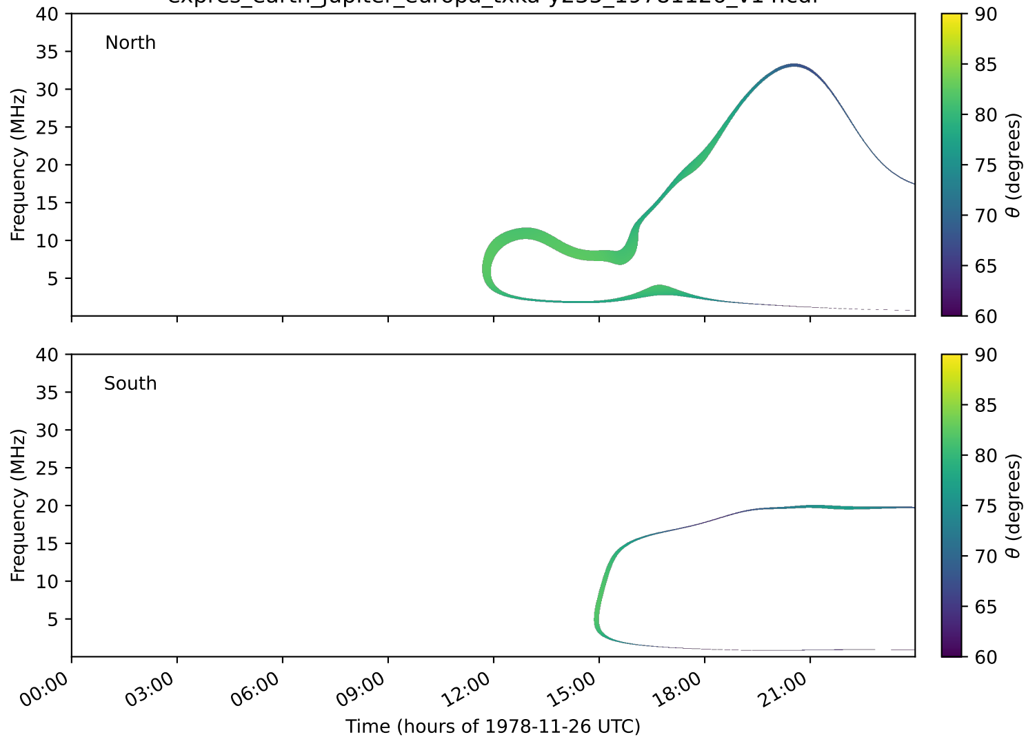
expres_earth_jupiter_europa_txka-y235_19781126_v14.cdf
