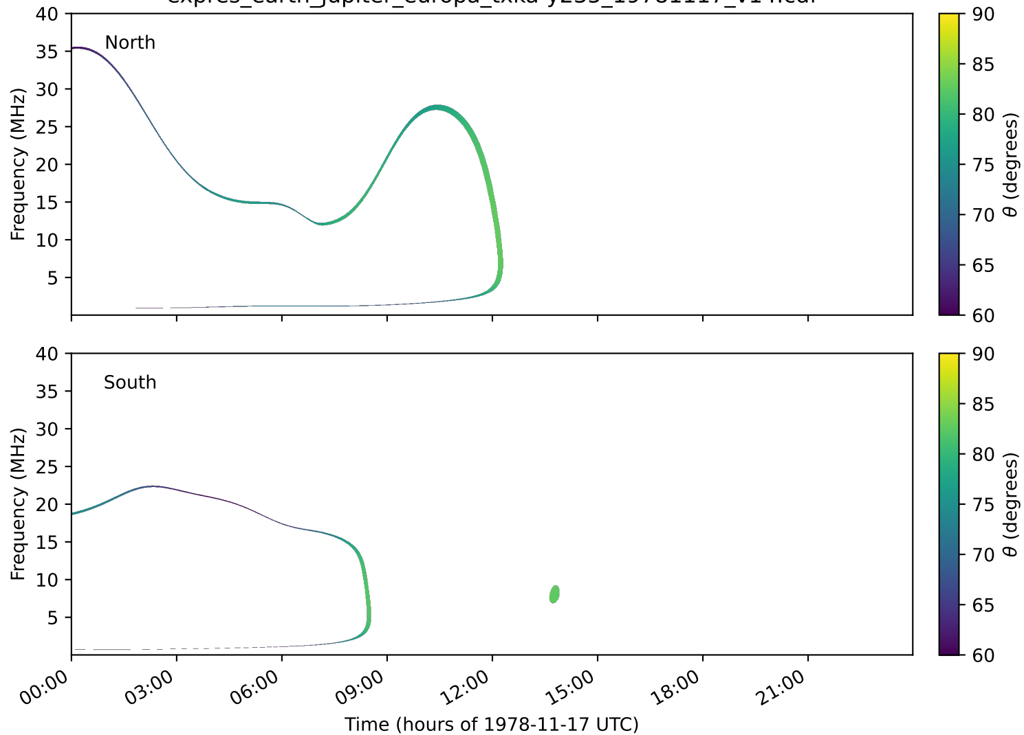
expres_earth_jupiter_europa_txka-y235_19781117_v14.cdf
