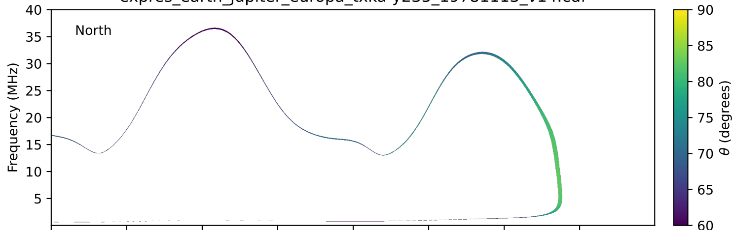
expres_earth_jupiter_europa_txka-y235_19781113_v14.cdf
