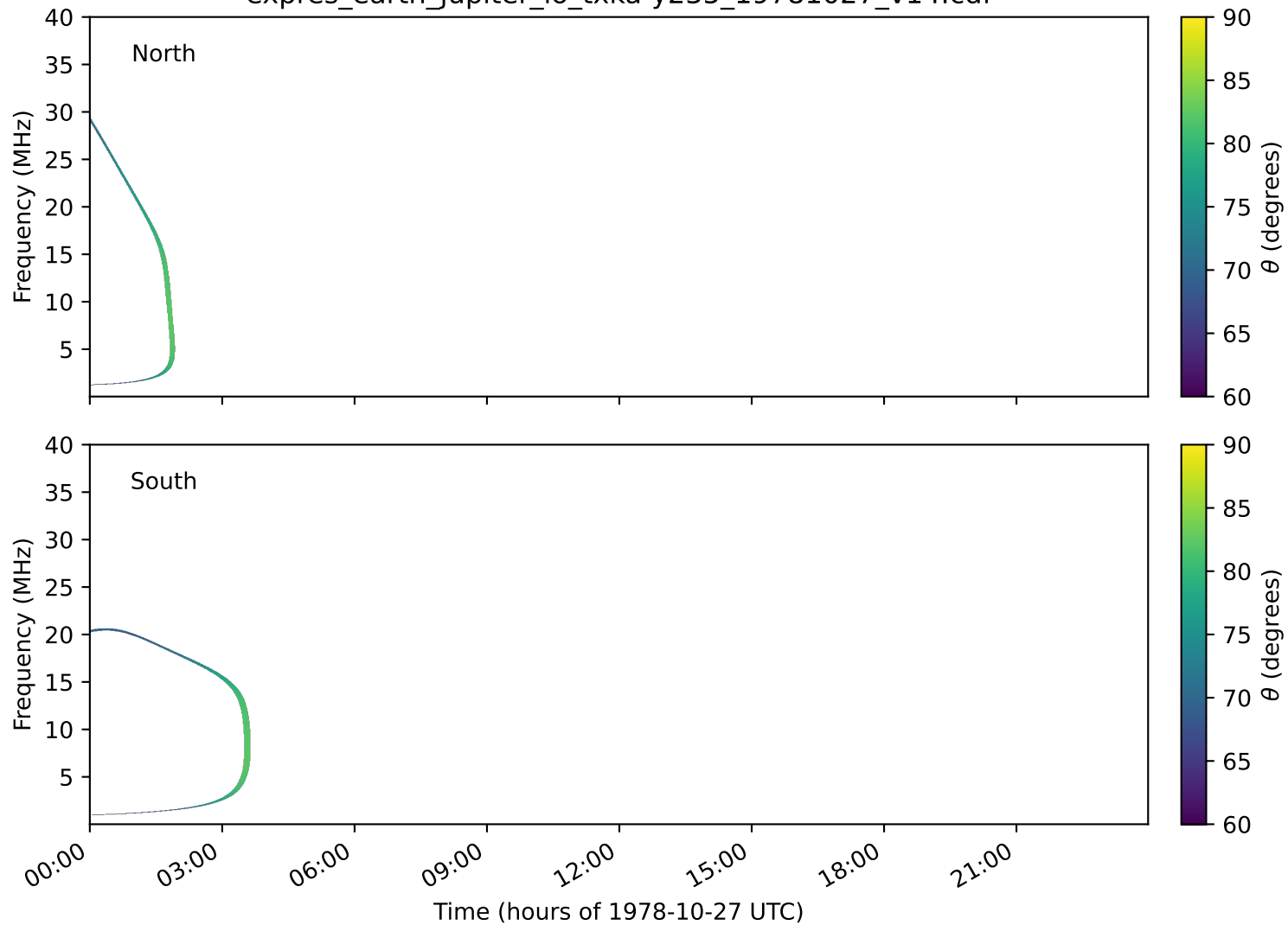
expres_earth_jupiter_io_txka-y235_19781027_v14.cdf
