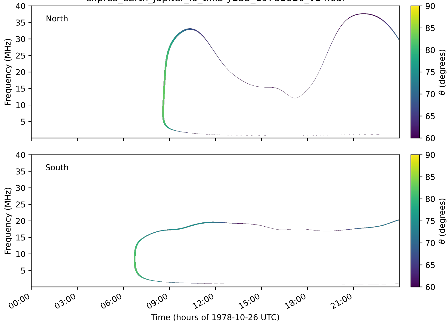
expres_earth_jupiter_io_txka-y235_19781026_v14.cdf
