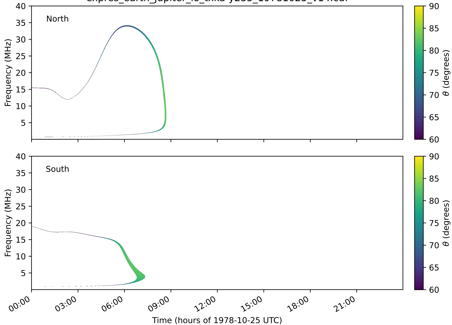
expres_earth_jupiter_io_txka-y235_19781025_v14.cdf
