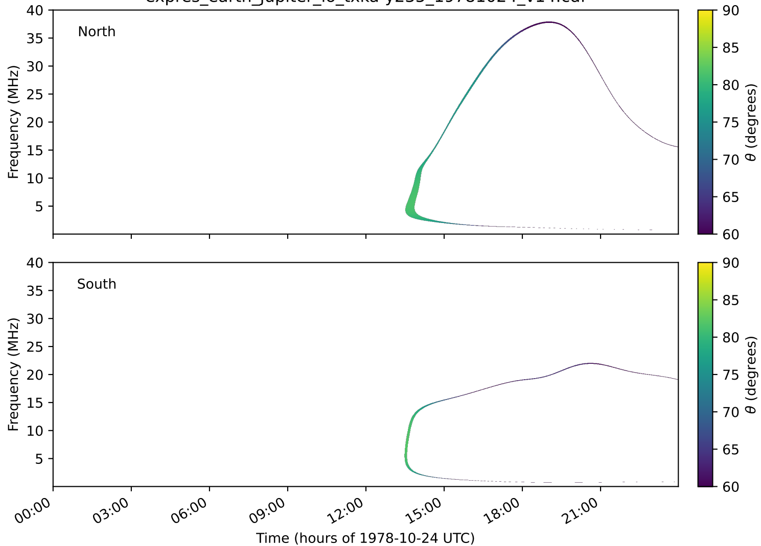
expres_earth_jupiter_io_txka-y235_19781024_v14.cdf
