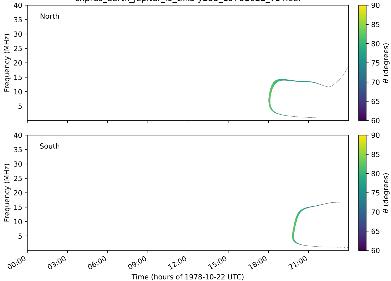
expres_earth_jupiter_io_txka-y235_19781022_v14.cdf
