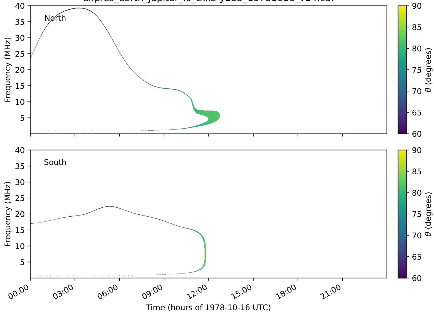
expres_earth_jupiter_io_txka-y235_19781016_v14.cdf
