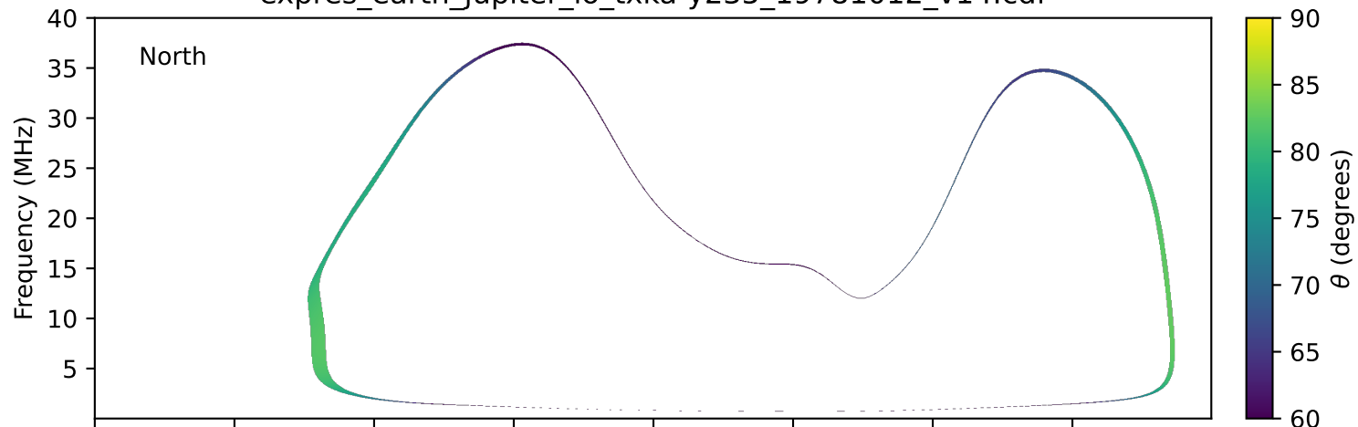
expres_earth_jupiter_io_txka-y235_19781012_v14.cdf
