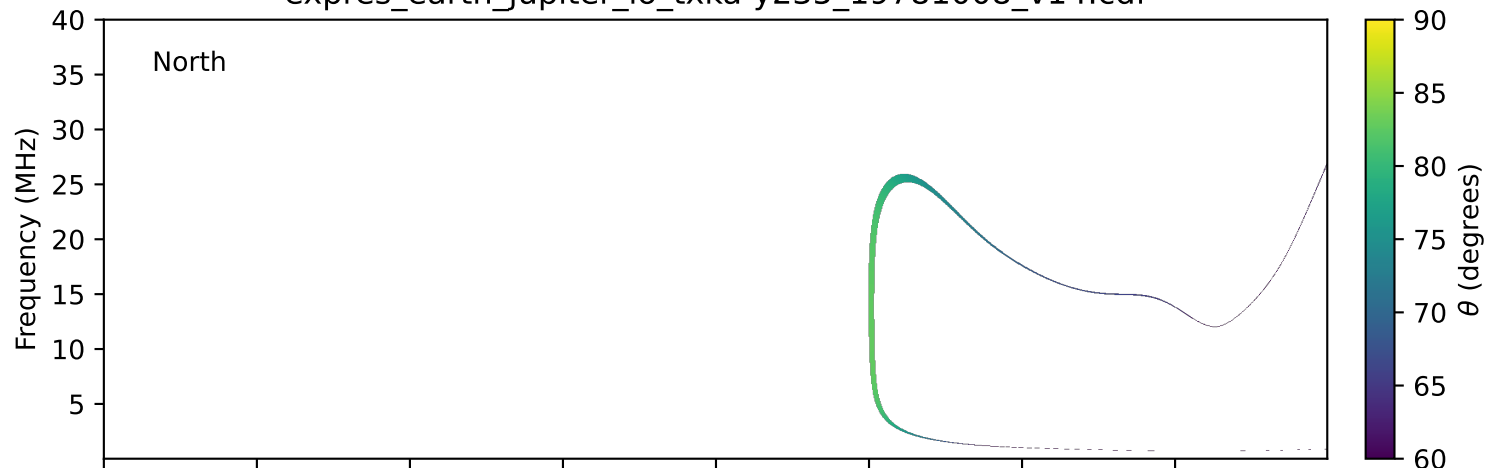
expres_earth_jupiter_io_txka-y235_19781008_v14.cdf
