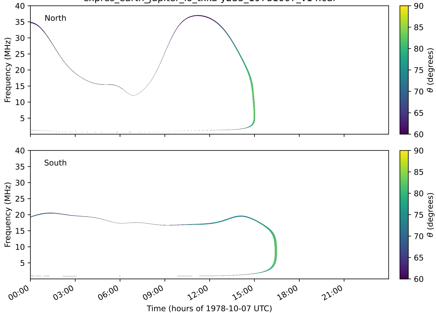
expres_earth_jupiter_io_txka-y235_19781007_v14.cdf
