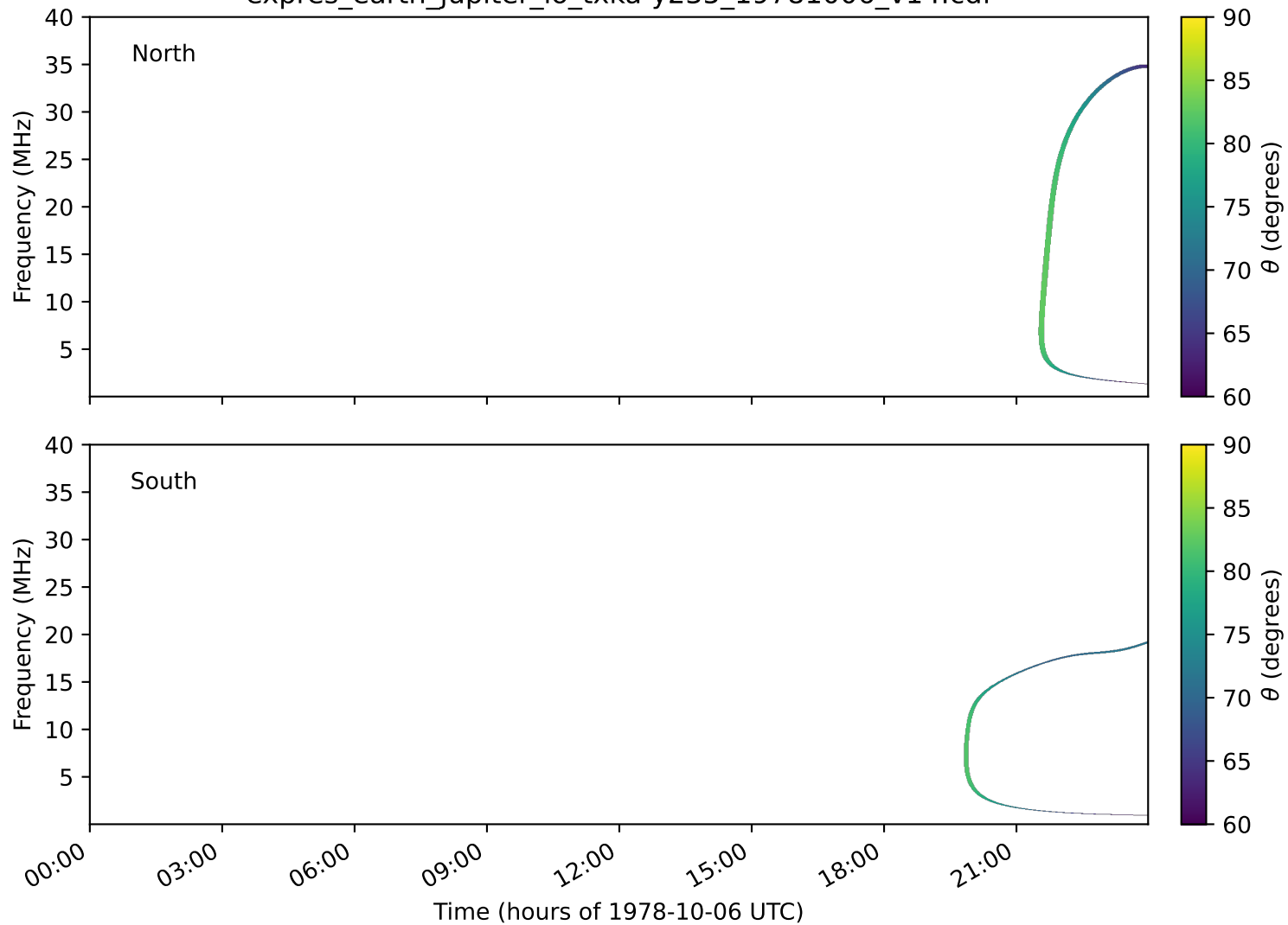
expres_earth_jupiter_io_txka-y235_19781006_v14.cdf
