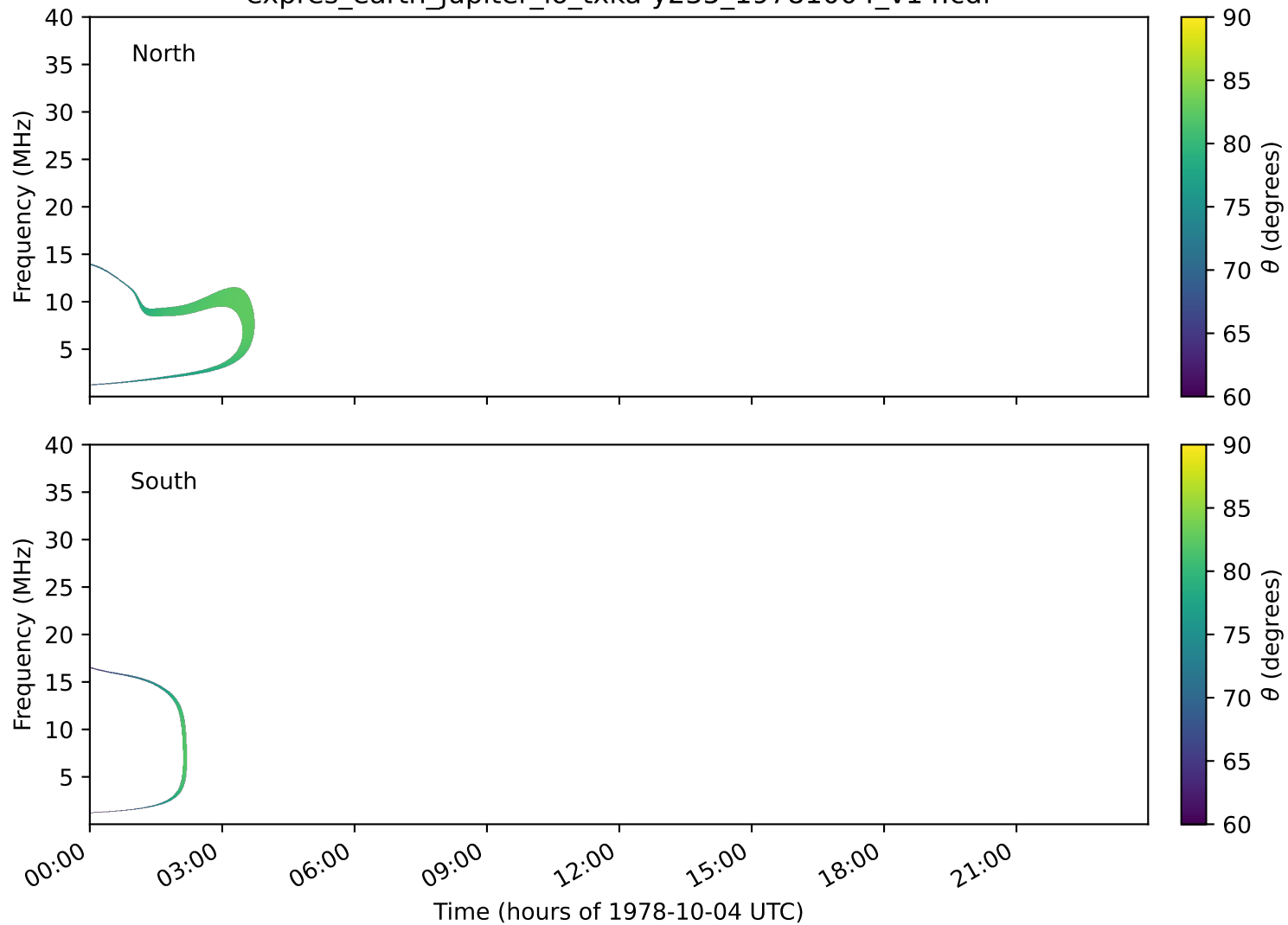
expres_earth_jupiter_io_txka-y235_19781004_v14.cdf
