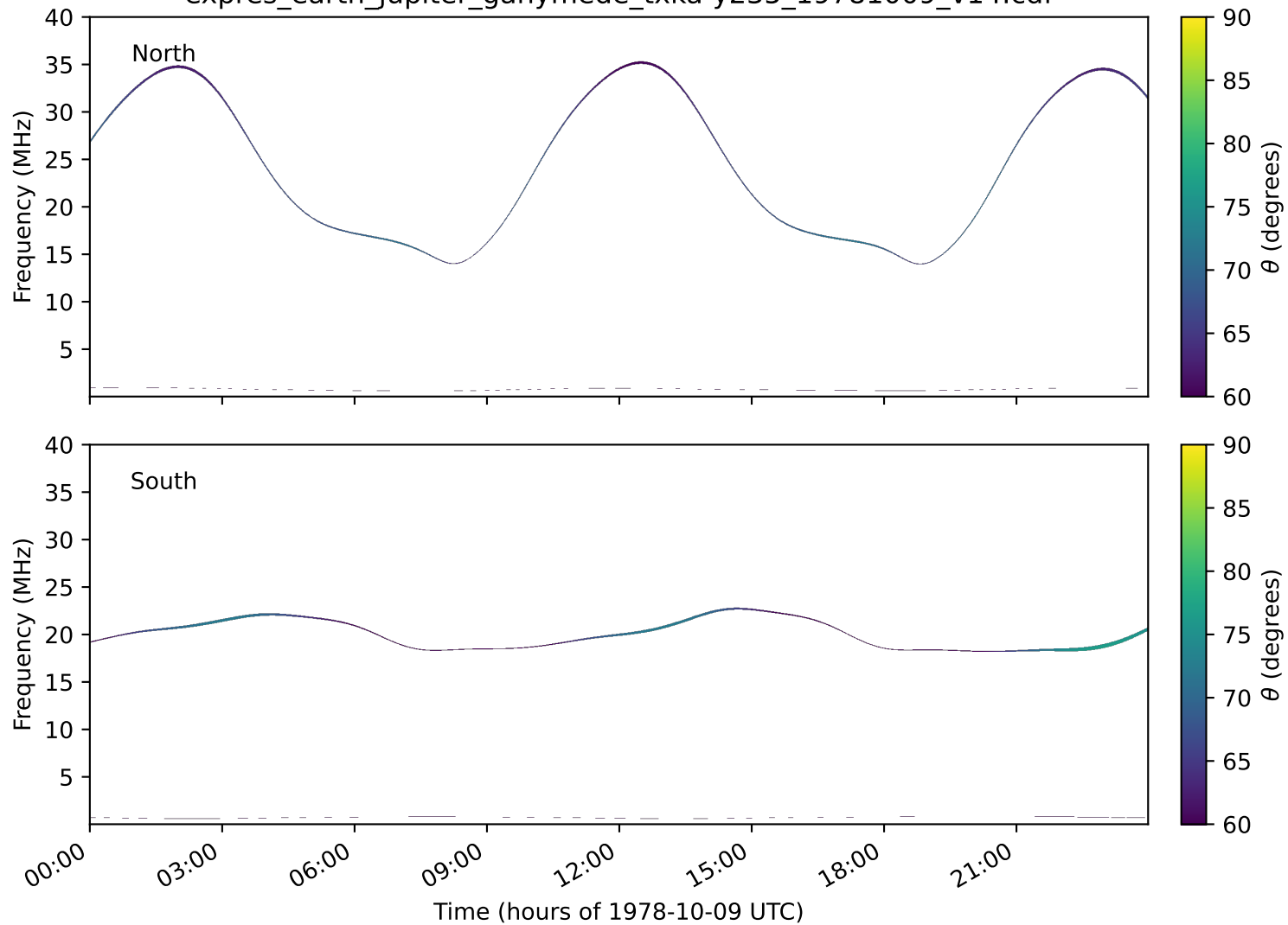
expres_earth_jupiter_ganymede_txka-y235_19781009_v14.cdf
