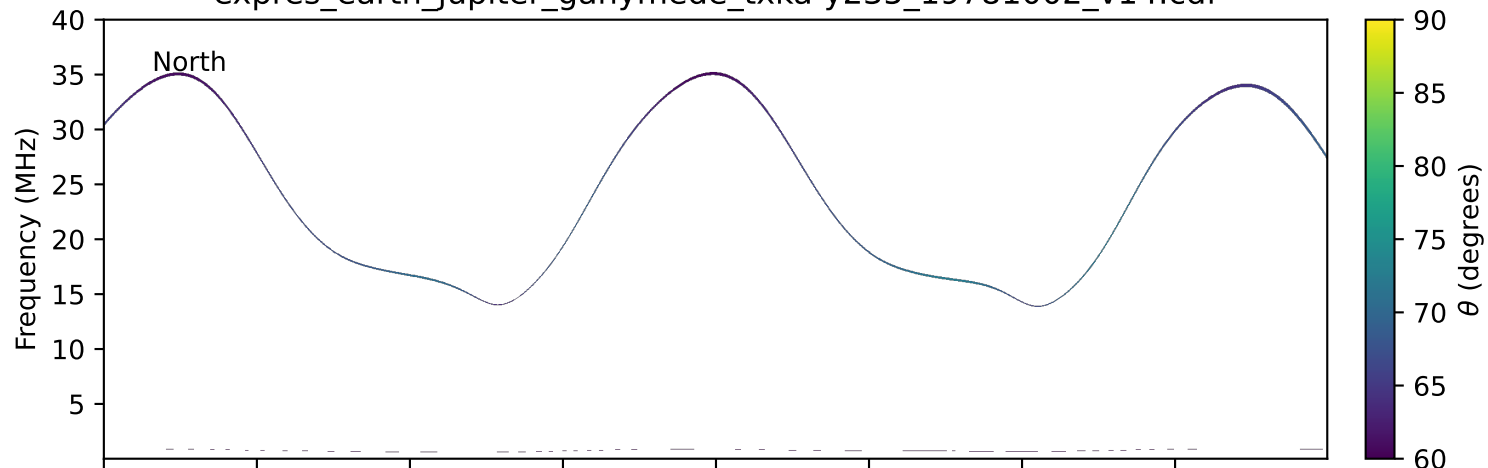
expres_earth_jupiter_ganymede_txka-y235_19781002_v14.cdf
