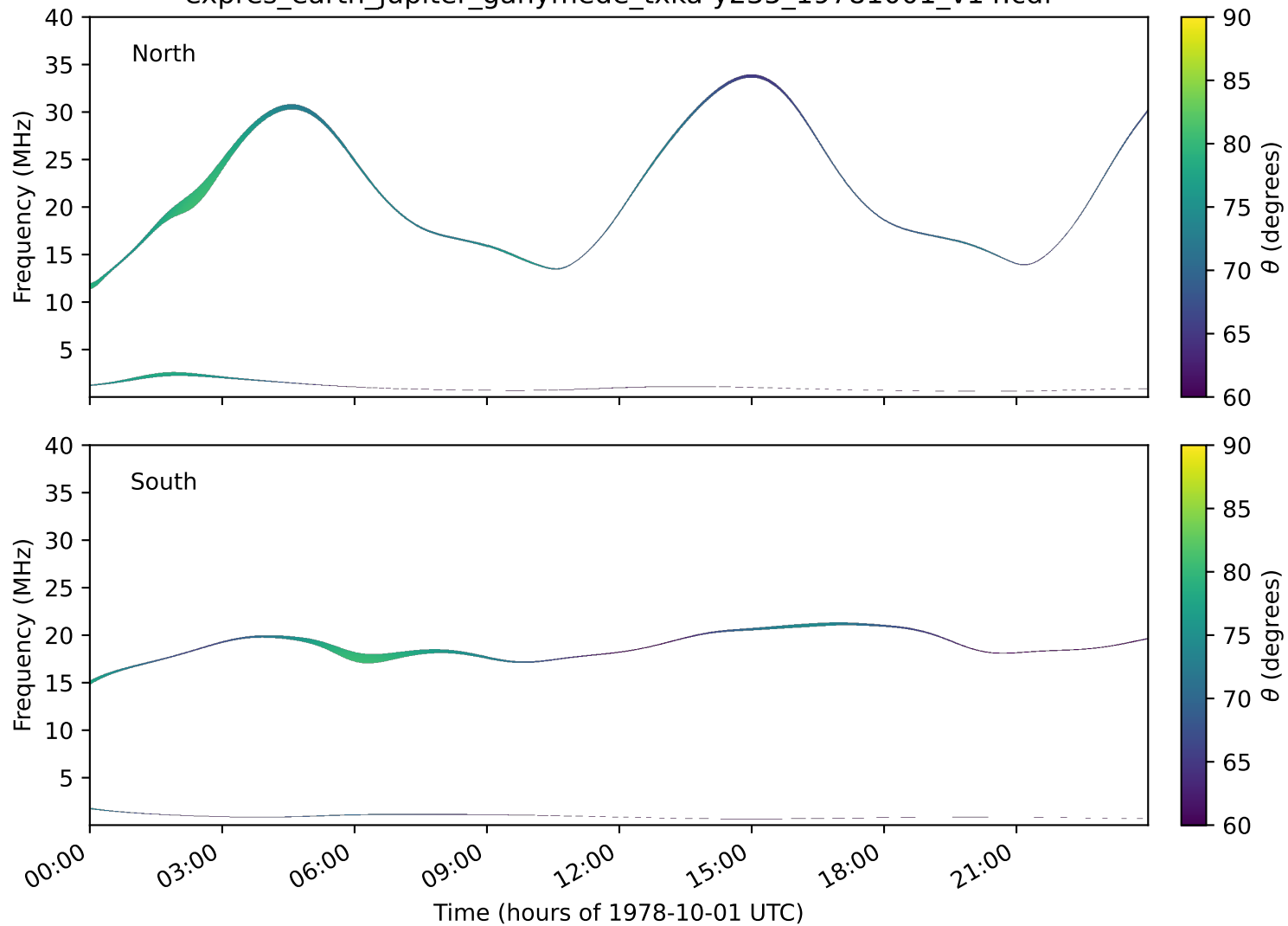
expres_earth_jupiter_ganymede_txka-y235_19781001_v14.cdf
