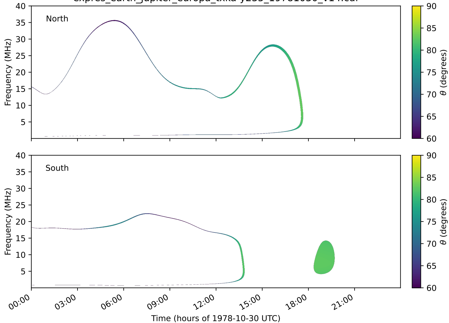
expres_earth_jupiter_europa_txka-y235_19781030_v14.cdf
