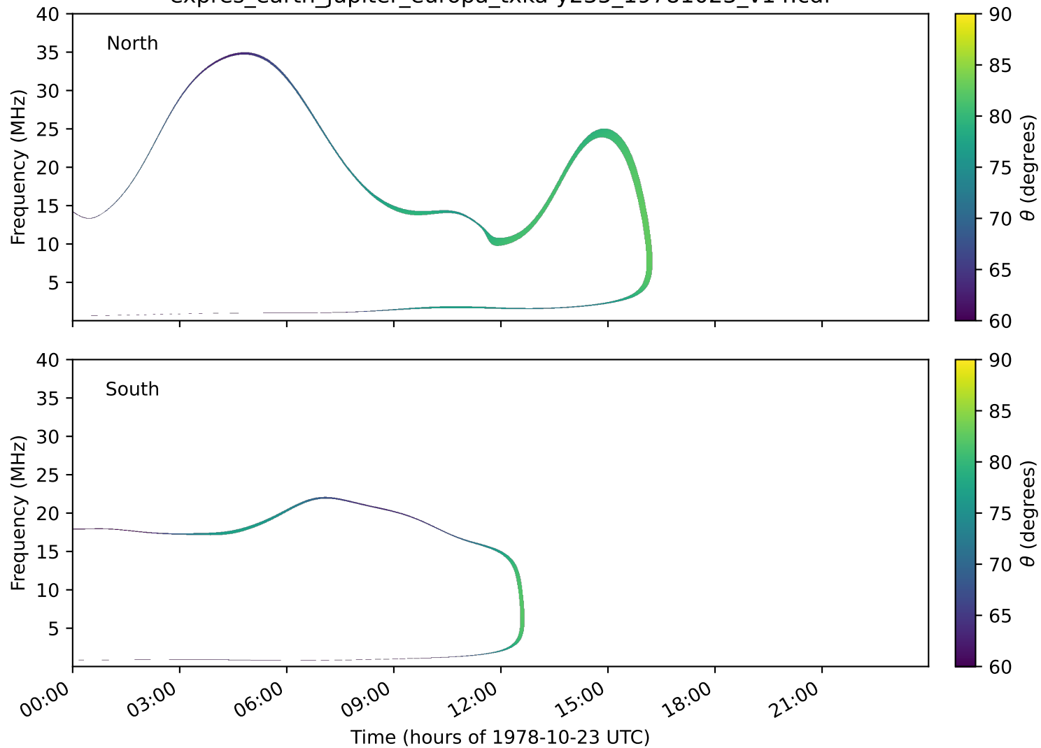
expres_earth_jupiter_europa_txka-y235_19781023_v14.cdf
