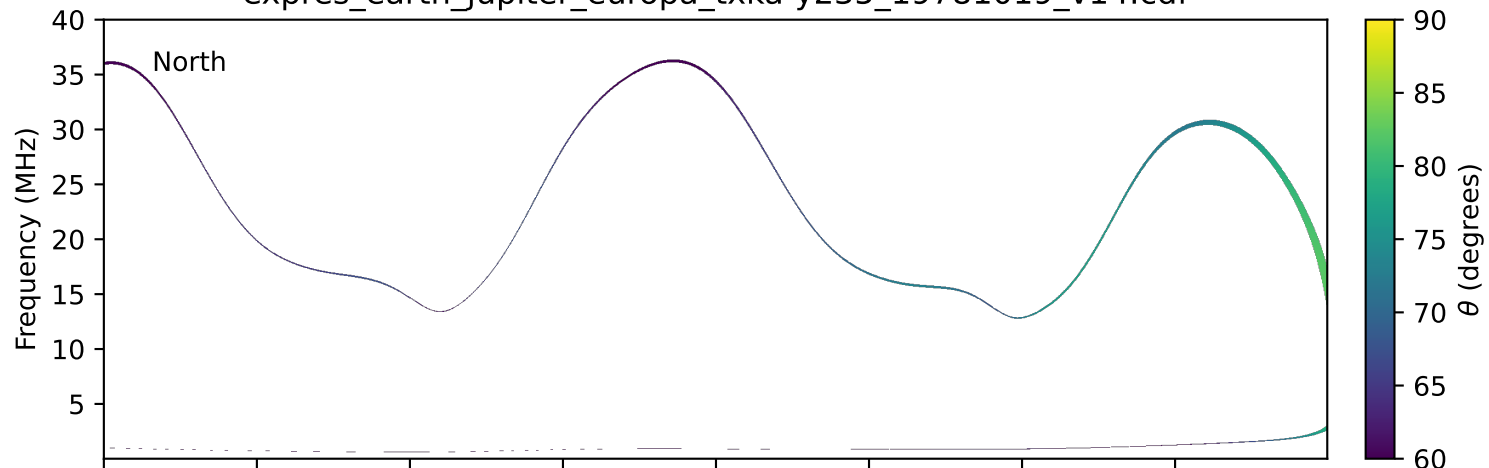
expres_earth_jupiter_europa_txka-y235_19781019_v14.cdf
