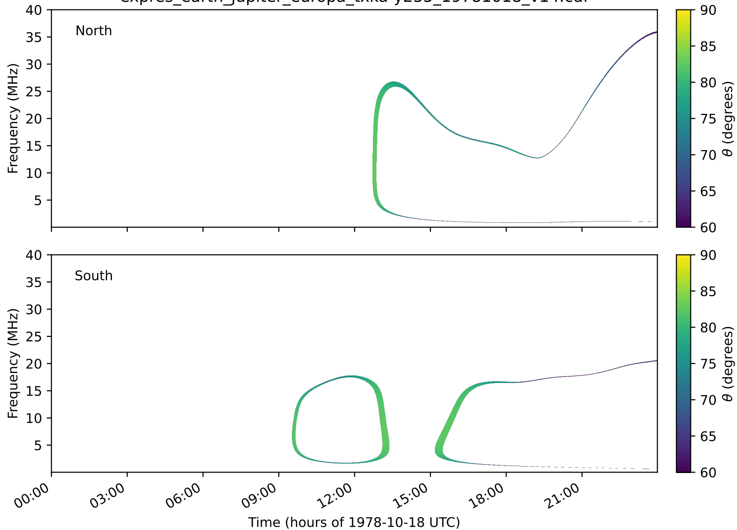
expres_earth_jupiter_europa_txka-y235_19781018_v14.cdf
