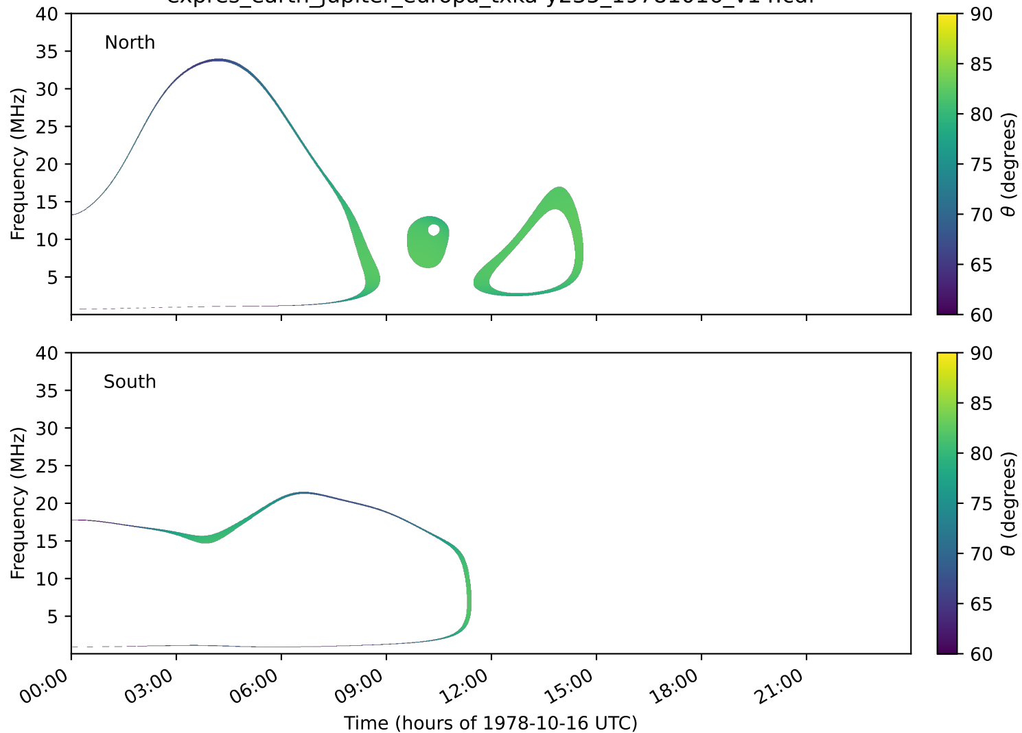
expres_earth_jupiter_europa_txka-y235_19781016_v14.cdf
