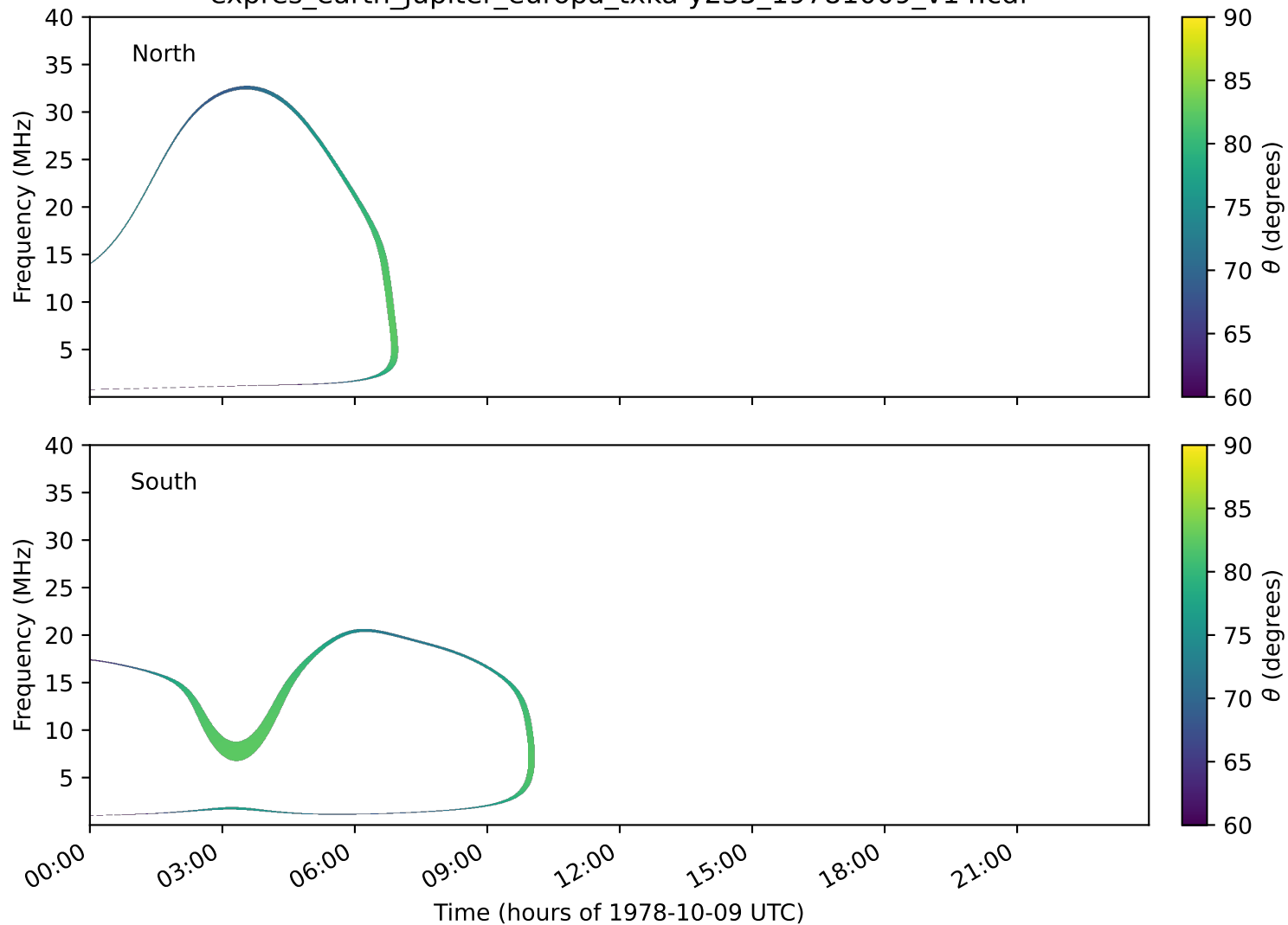
expres_earth_jupiter_europa_txka-y235_19781009_v14.cdf
