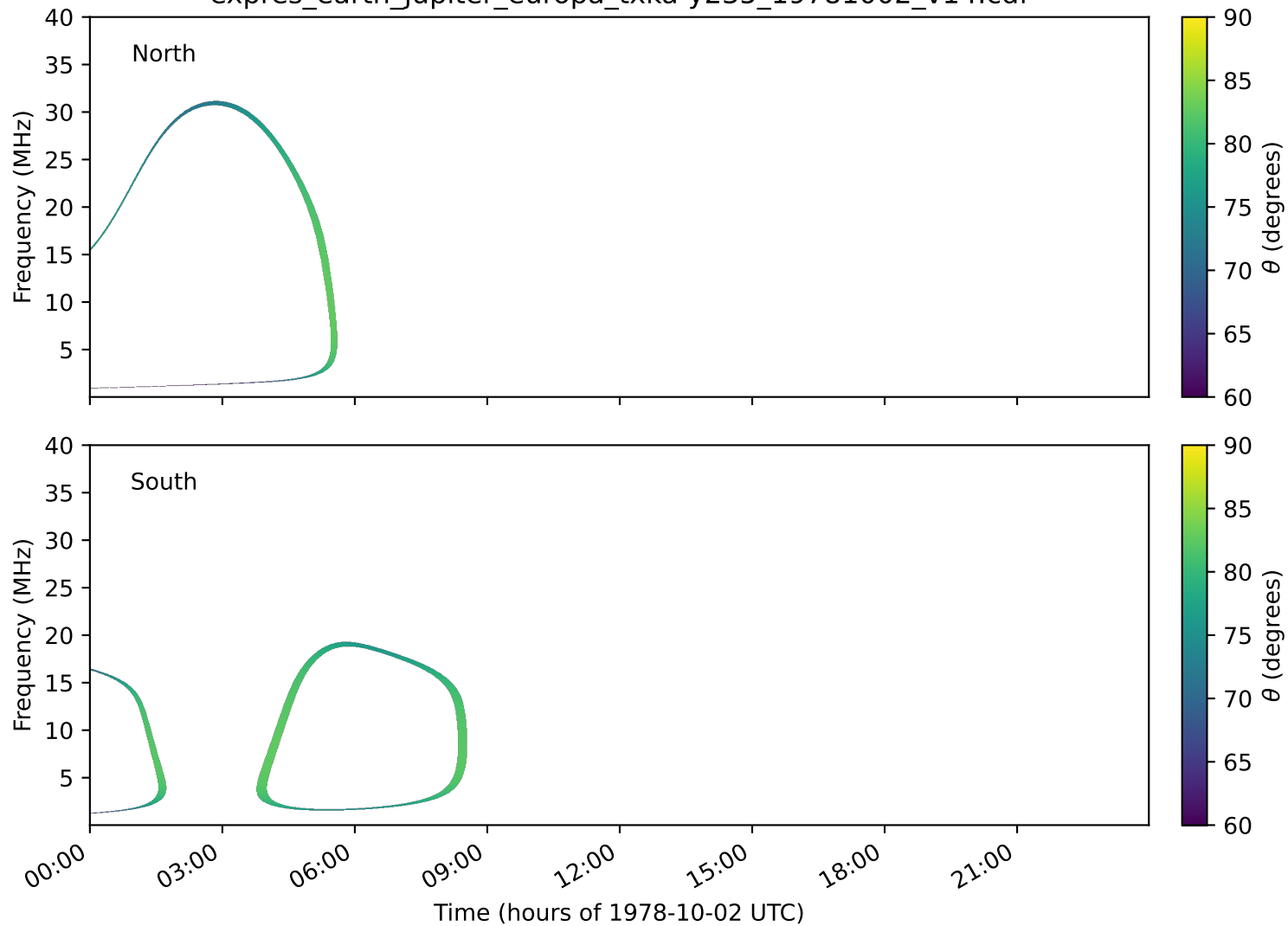
expres_earth_jupiter_europa_txka-y235_19781002_v14.cdf
