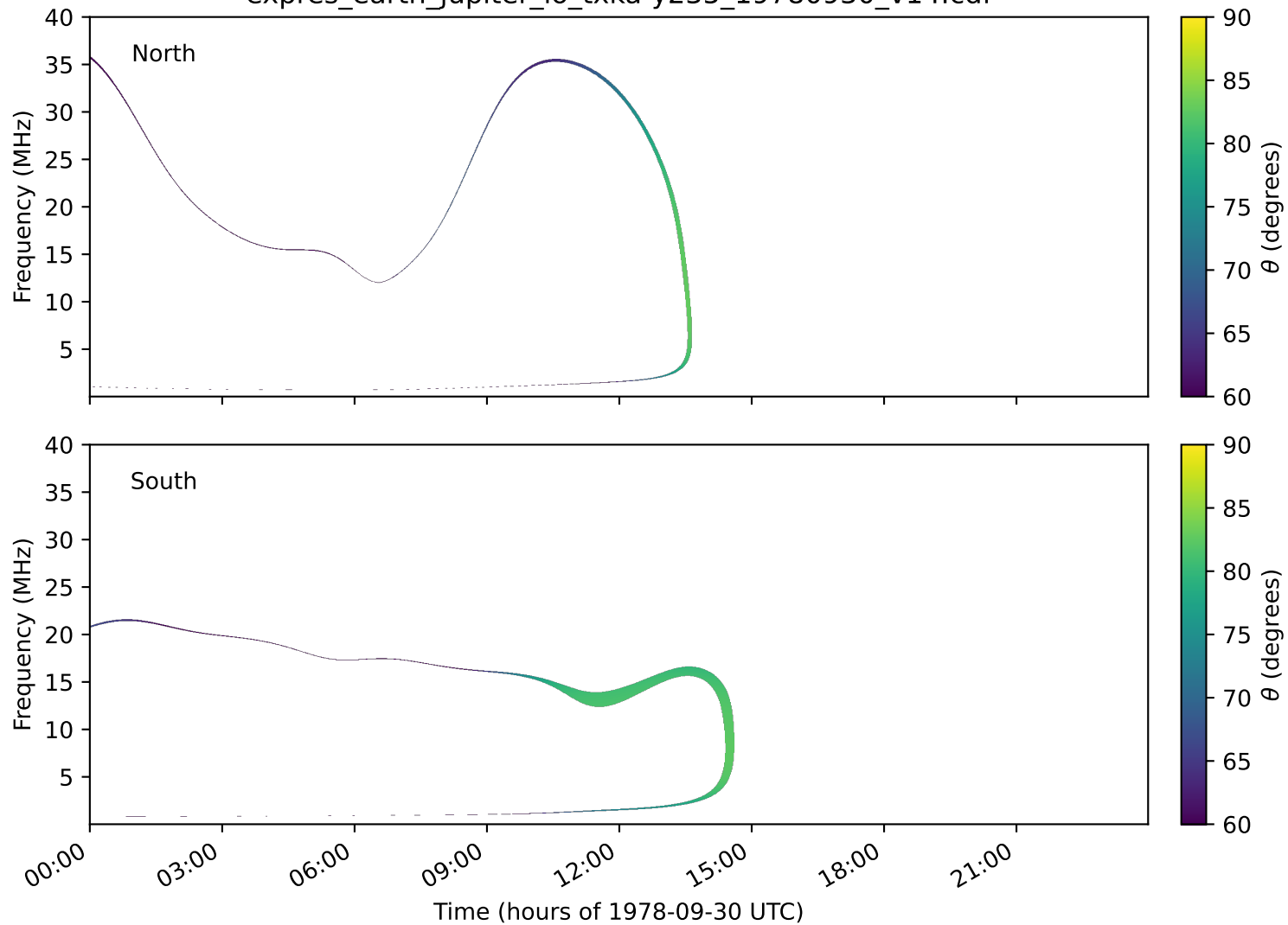
expres_earth_jupiter_io_txka-y235_19780930_v14.cdf
