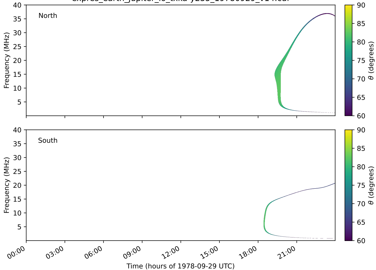
expres_earth_jupiter_io_txka-y235_19780929_v14.cdf
